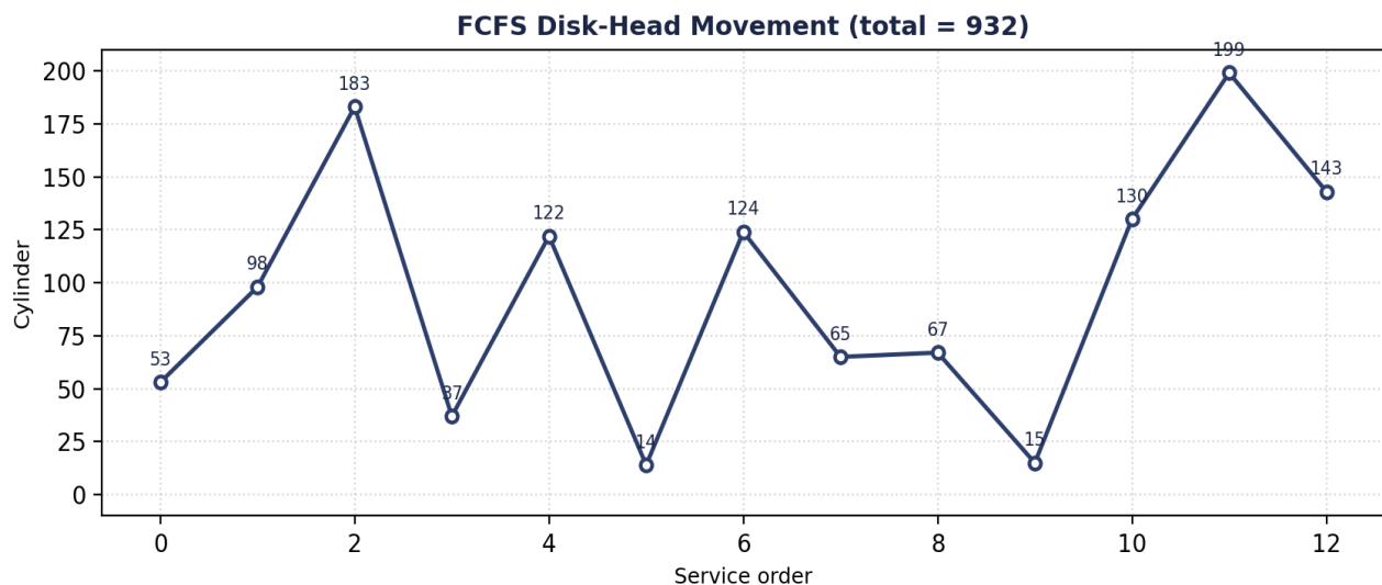
Figure 5.4 — FCFS head movement: 932 cylinders total (actual simulation output).
