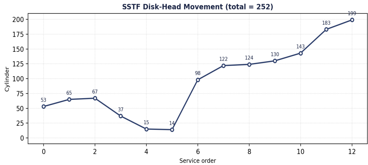
Figure 5.5 — SSTF head movement: 252 cylinders total — the lowest of all four algorithms (actual simulation output).
