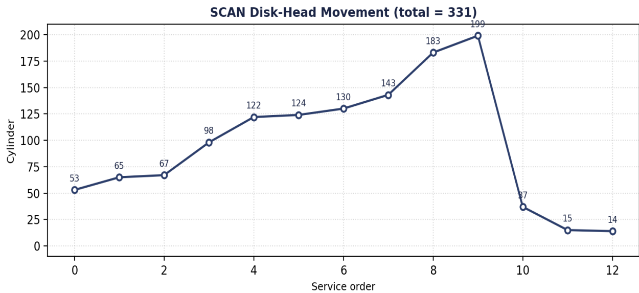
Figure 5.6 — SCAN head movement: 331 cylinders total — UniCore's recommended production algorithm (actual simulation output).
