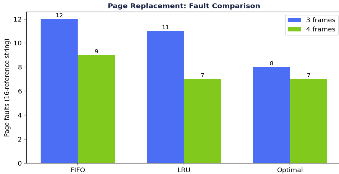
Figure 5.3 — FIFO vs LRU vs Optimal page faults on the 16-reference UniCore workload, at 3 and 4 frames (actual simulation output).
