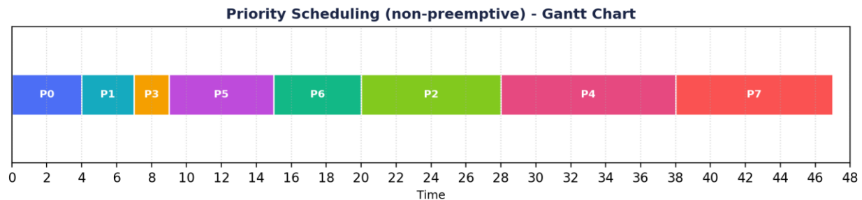
Figure 5.1 — Priority Scheduling (non-preemptive) Gantt chart (actual simulation output).
