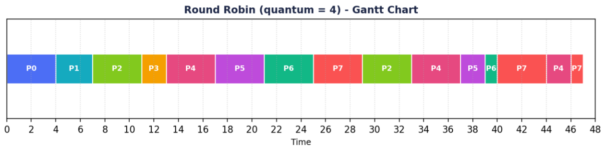
Figure 5.2 — Round Robin (quantum = 4) Gantt chart (actual simulation output).
